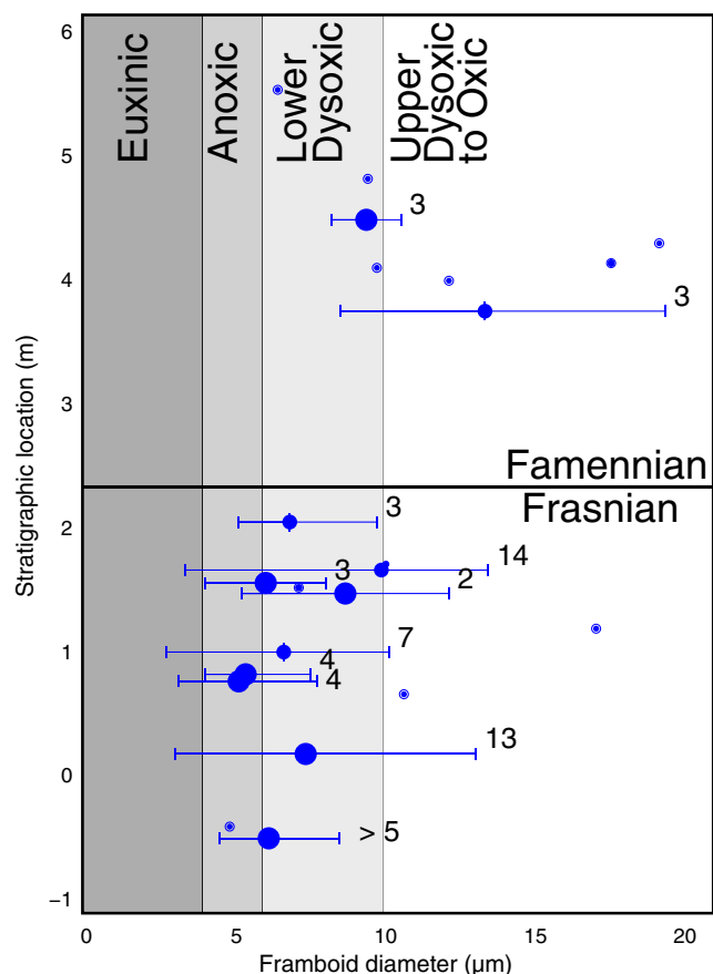
Fig. 11. The size and variability of pyrite framboids can be used to assess redox conditions (Wignall and Newton, 1998; Bond and Wignall, 2010). Euxinia produces populations of tiny framboids ( <5\ \mu\text{m} ) with a narrow size range. In dysoxic environments the framboids are larger and more variable in size ( 5\text{--}15\ \mu\text{m} ). Framboids are rare in oxic environments. The chart shows the distribution of framboids from SEM. Individual points indicate a single framboid in the sample. Lines show minimum, maximum and average size for the framboid population in that sample. Framboid populations are indicated for each large data point where n > 1 . Based on the framboid populations, the Upper Frasnian shows an anoxic to lower dysoxic environment consistent with the Kellwasser Anoxia Event. Framboids are much less abundant in the Famennian part of the section indicating a change to upper dysoxic to oxic environments. Stratigraphy is measured from the base of the Hongguleleng Formation.
